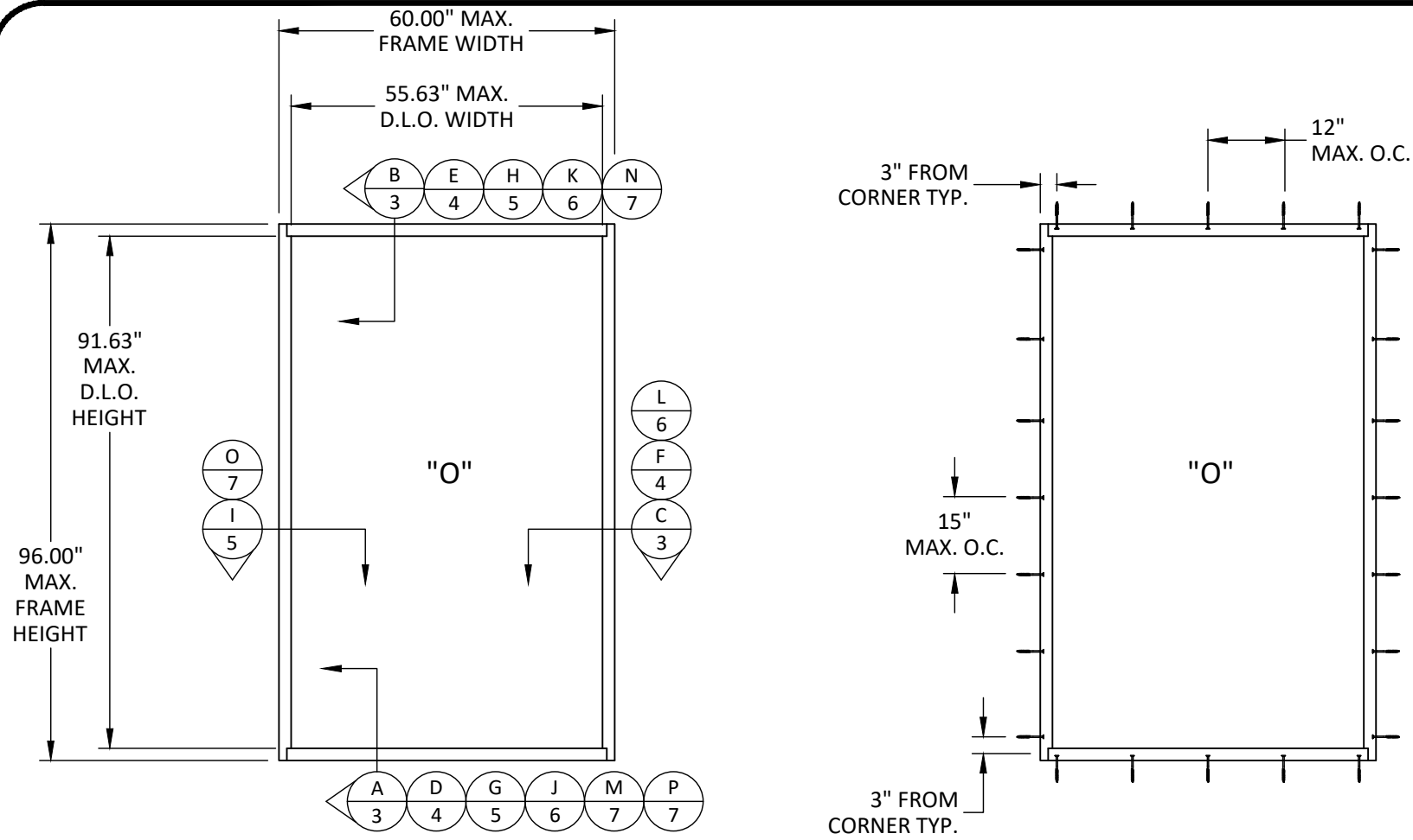
ANCHOR LAYOUT SINGLE UNITS
